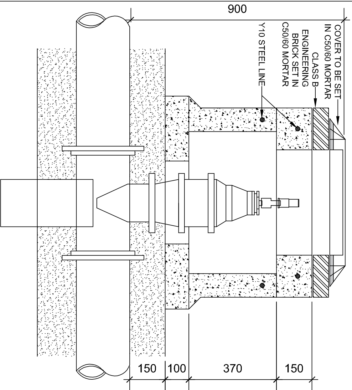
SECTION VIEW: UNTRAFFICED MIN. 900mm.
