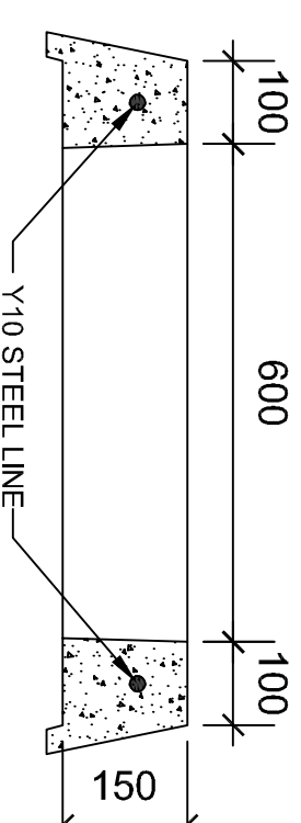
RISER SECTION VIEW
