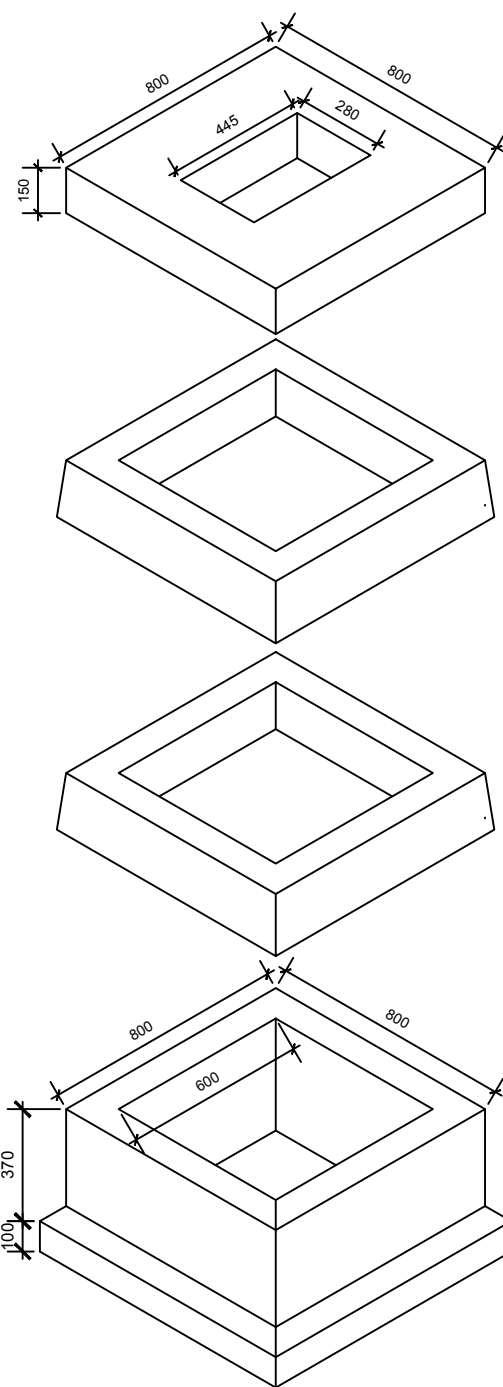
BASE AND CHAMBER CAST MONOLITHIC
