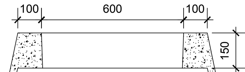
RISER SECTION VIEW
