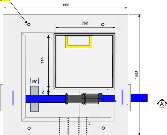
PLAN VIEW: BULK WATER METER
