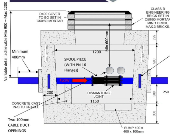
SECTION A-A: BULK WATER METER
