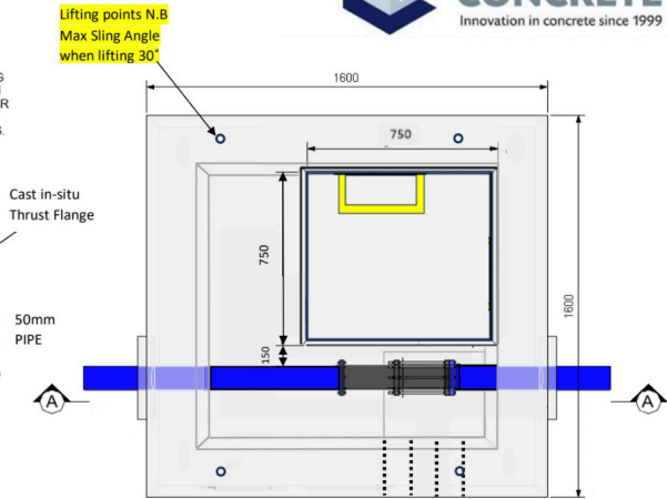
PLAN VIEW: BULK WATER METER
