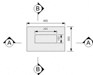
PLAN VIEW: MARKER POST COMPLETE WITH CONCRETE SURROUND
