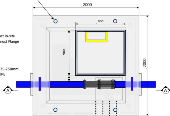
PLAN VIEW: BULK WATER METER
