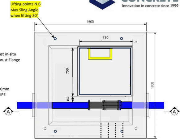
PLAN VIEW: BULK WATER METER
