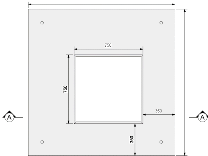
PLAN VIEW:
