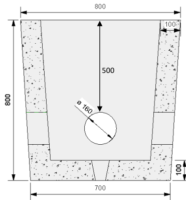
SECTION VIEW A-A:
