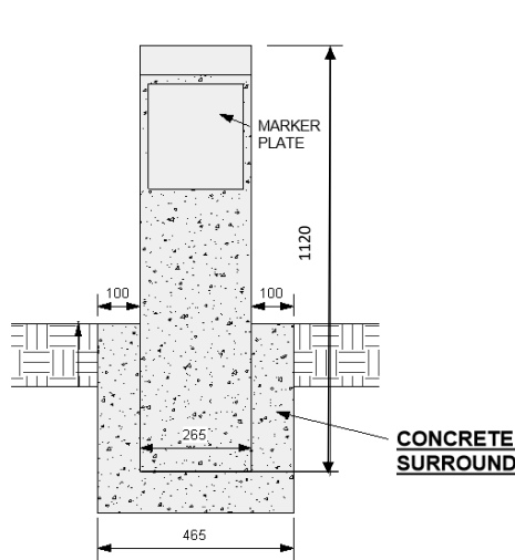
SECTION A-A: MARKER POST COMPLETE WITH CONCRETE SURROUND
