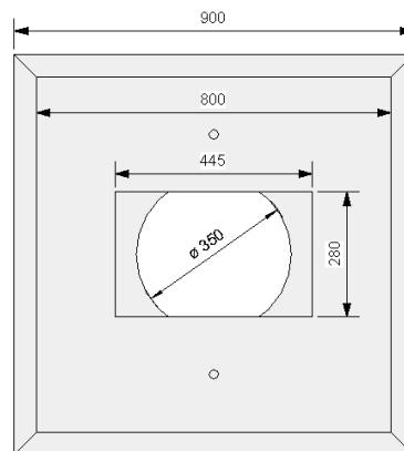
PLAN VIEW WITH COVER OPENING 445 X 280MM
